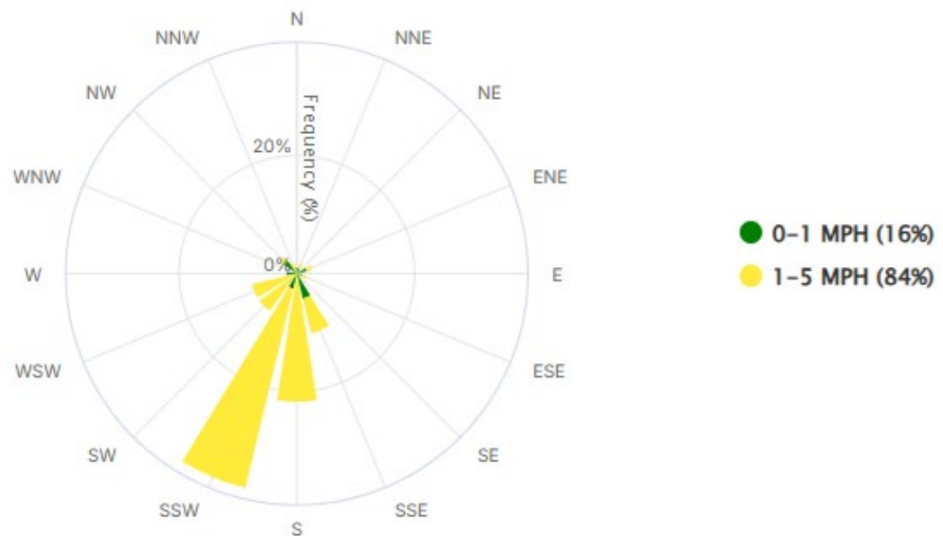
Figure 3 CM6 – Focus Points Wind Rose August 1, 2025, 2:17 PM to 4:16 PM
