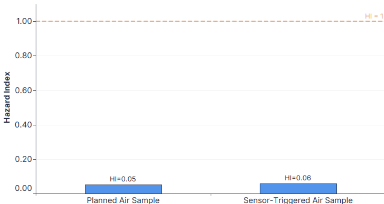
Figure 5 Hazard Indices at the CCND CM6 – Focus Points for Planned (August 27, 2025) and Sensor-Triggered (August 1, 2025) Air Samples
